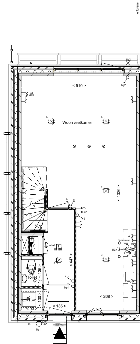
00 begane grond
